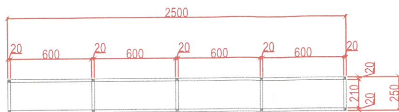
Floor Plan Details
