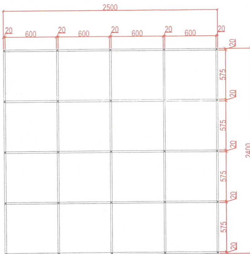
Front Elevation Details
